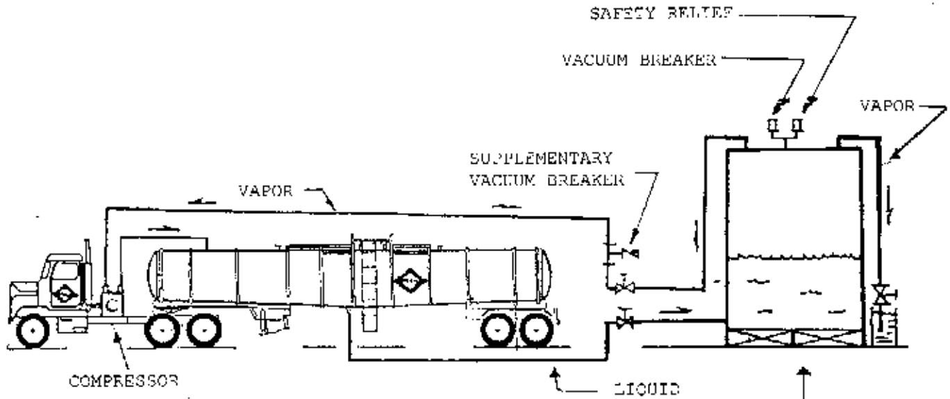
COMPRESSOR METHOD
